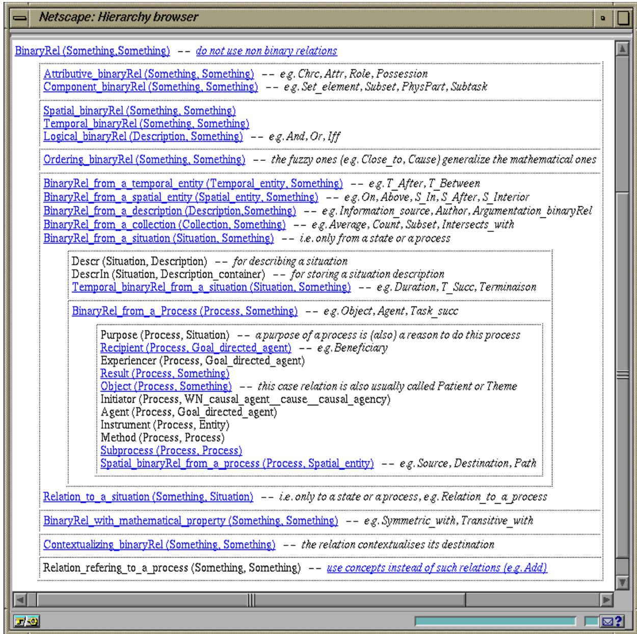
Fig. 6. Uppermost relation types of the WebKB top-level ontology as shown by the WebKB hierarchy browser (types at the same level in a same box are exclusive - i.e. cannot have common subtypes - but are not exclusive with types in other boxes).
