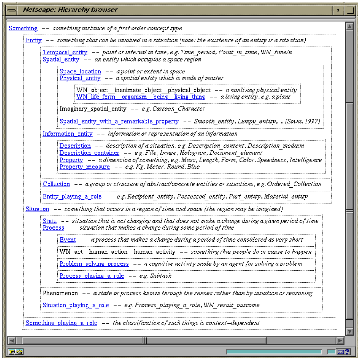
Fig. 7. Uppermost concept types of the WebKB top-level ontology (types at the same level in a same box are exclusive; types beginning by WN come from the WordNet ontology).
