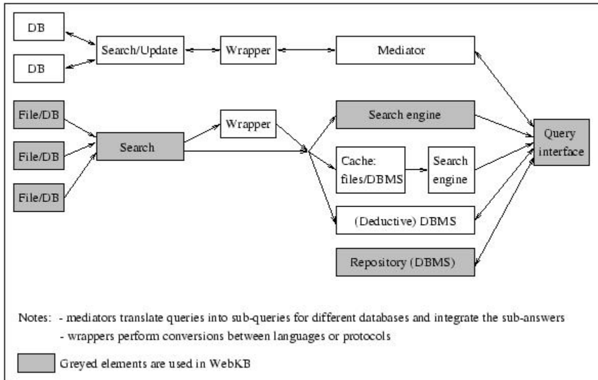
Fig. 1. Generalized architecture elements of Web-based IR/KA/Groupware systems.
