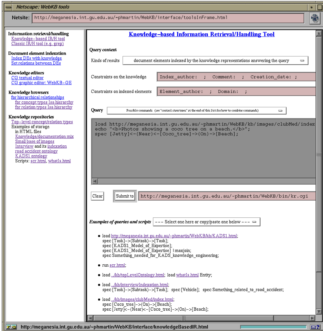
Fig. 2. The WebKB menu and knowledge-based Information Retrieval/Handling Tool. The example query shows how a document containing CGs (indexing images) is loaded into the WebKB processor and then how the command "spec" (which looks for specializations of a CG) can be used to retrieve CGs and the images they index. According to the value selected in the "kinds of results" option (cf. top right of the figure), the images, but not the knowledge statements, will be presented. A similar query and its results is shown in the figures 3 and 5.
