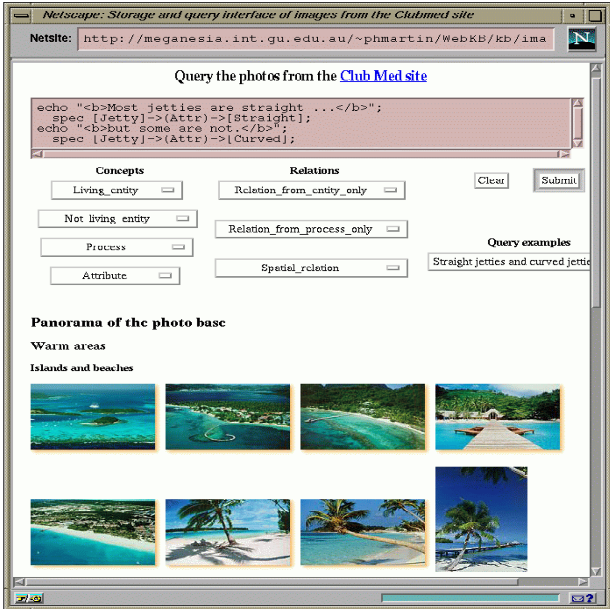
Fig. 3. Images, indexation and a customized query interface within the same document (the example query shows how the command "spec" can be used to retrieve images indexed by CGs. See the results in Figure 5).
