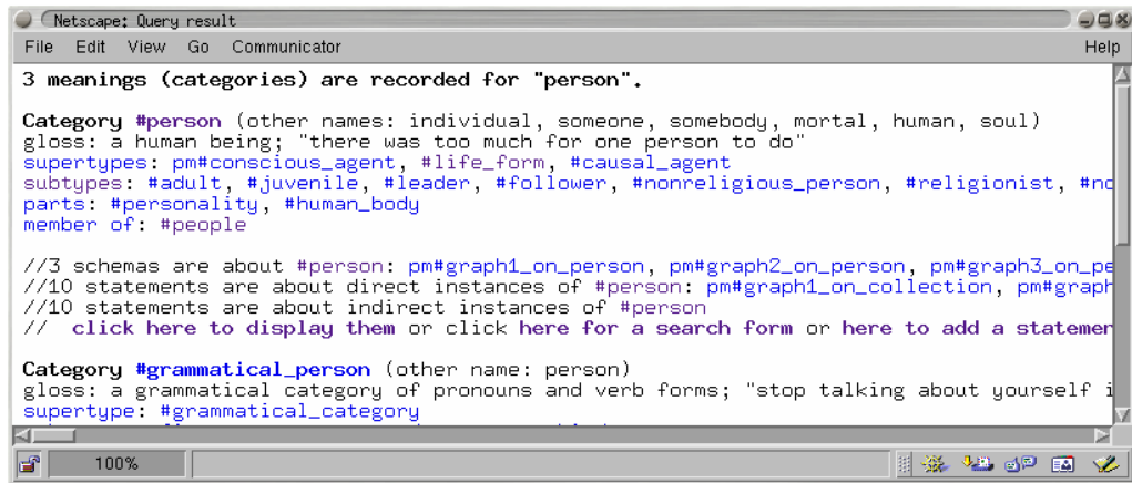
Fig. 3. Result of the previous query (Fig. 1) for “novice users”.
